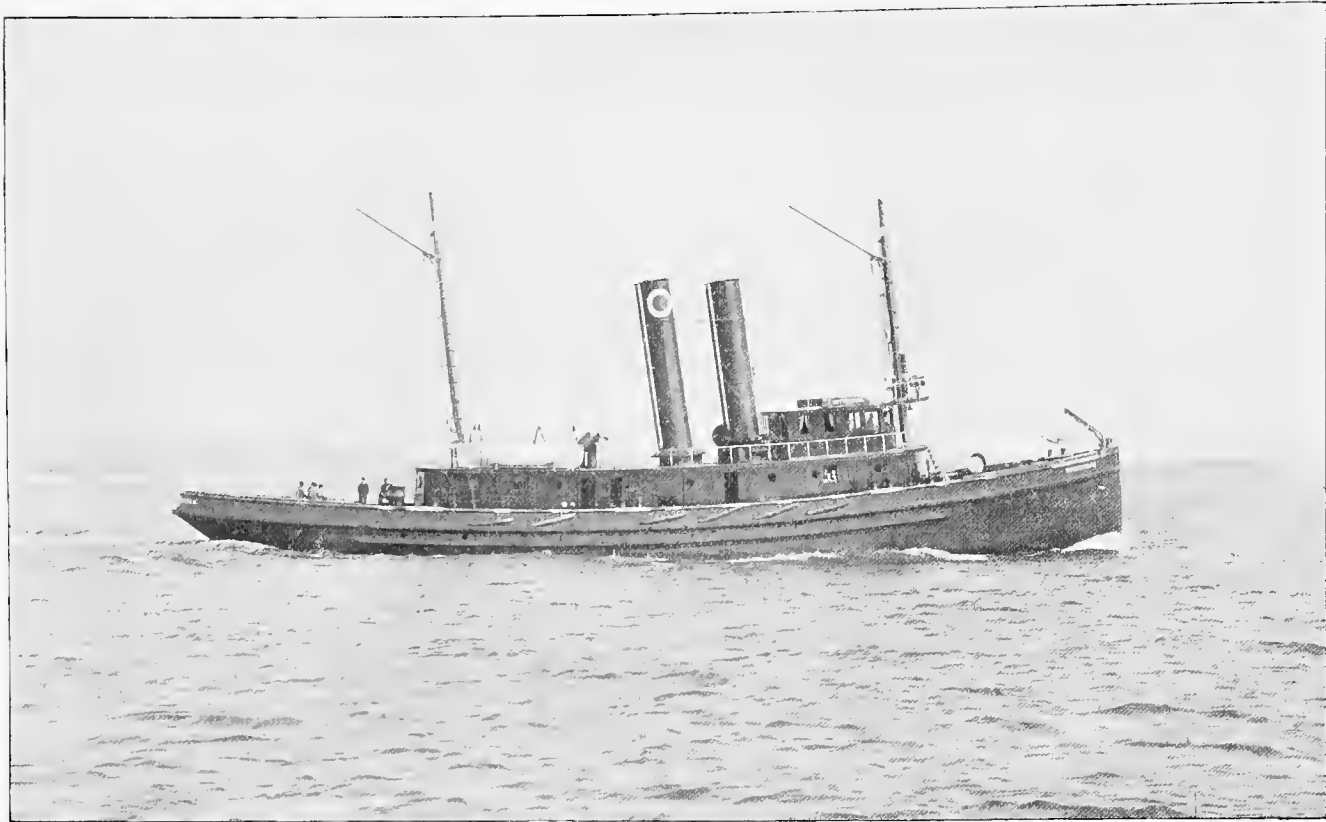
THE SEA-GOING STEEL TUG NOTTINGHAM.—Built by John H. Dialogue & Son, Camden, N. J.
